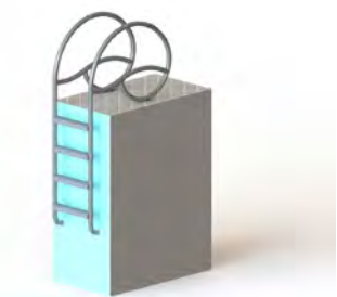
134640-02-.065 2 STEP SOLARIAN 30" LADDER 134640-03-.065 3 STEP SOLARIAN 30" LADDER 134640-04-.065 4 STEP SOLARIAN 30" LADDER
