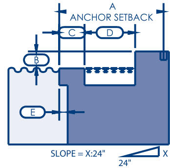
TROUGH GUTTER
