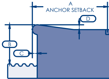
HAUNCH GUTTER
